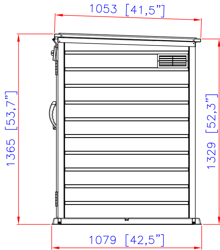
Side View
