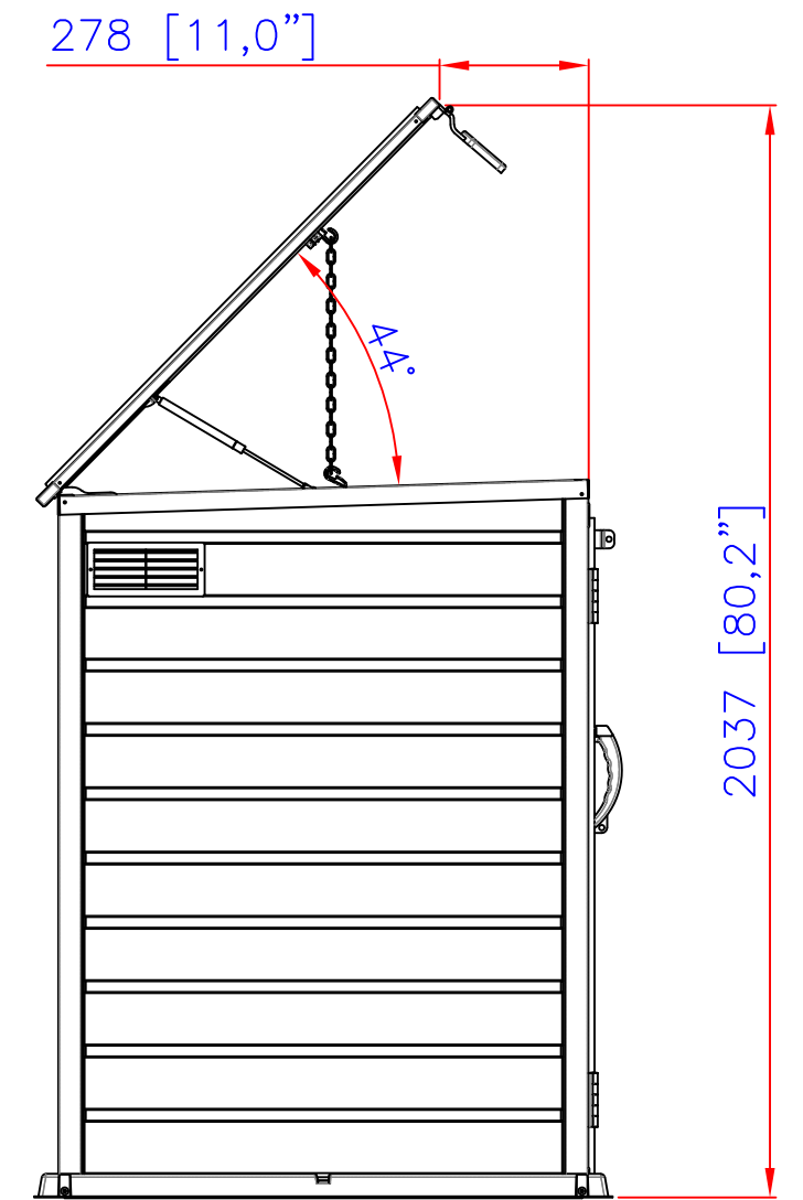
Top Lid Opened Side View
